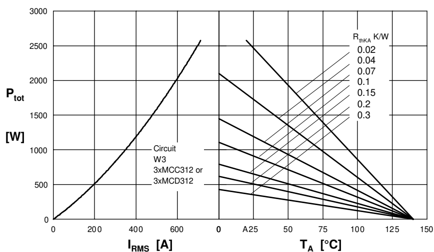
Fig. 8 Three phase AC-controller: Power dissipation versus R_{thJA} output current and ambient temperature
