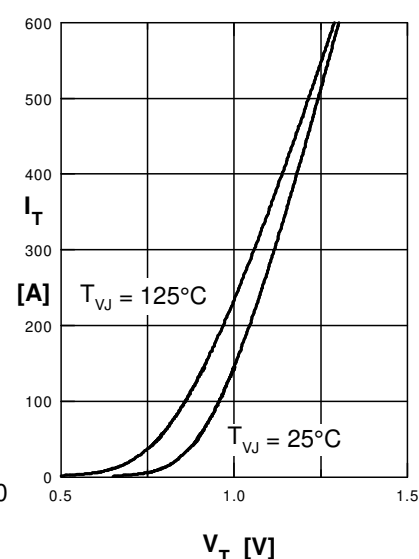
Fig. 9 Forward characteristics
